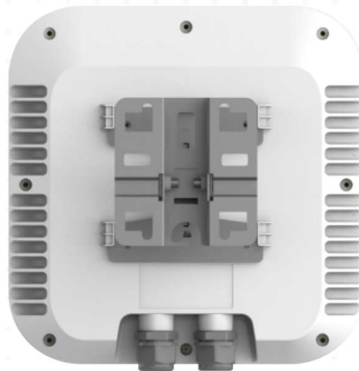
Figure 1-2 RG-RAP6260(G)
